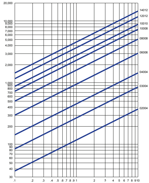
PRESSURE DROP P.S.I. WITH 1/32" OR LARGER SCREEN OPENING
